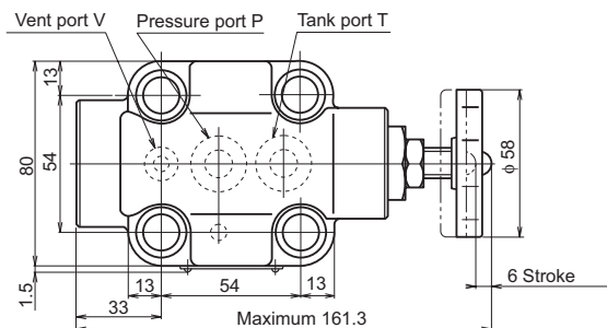
HDRI-G03: Gasket mount type
