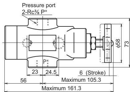
HDRI-T03: Screw connection type
